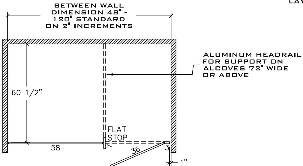
SINGLE ALCOVE (PILASTER SET @ 90°)
